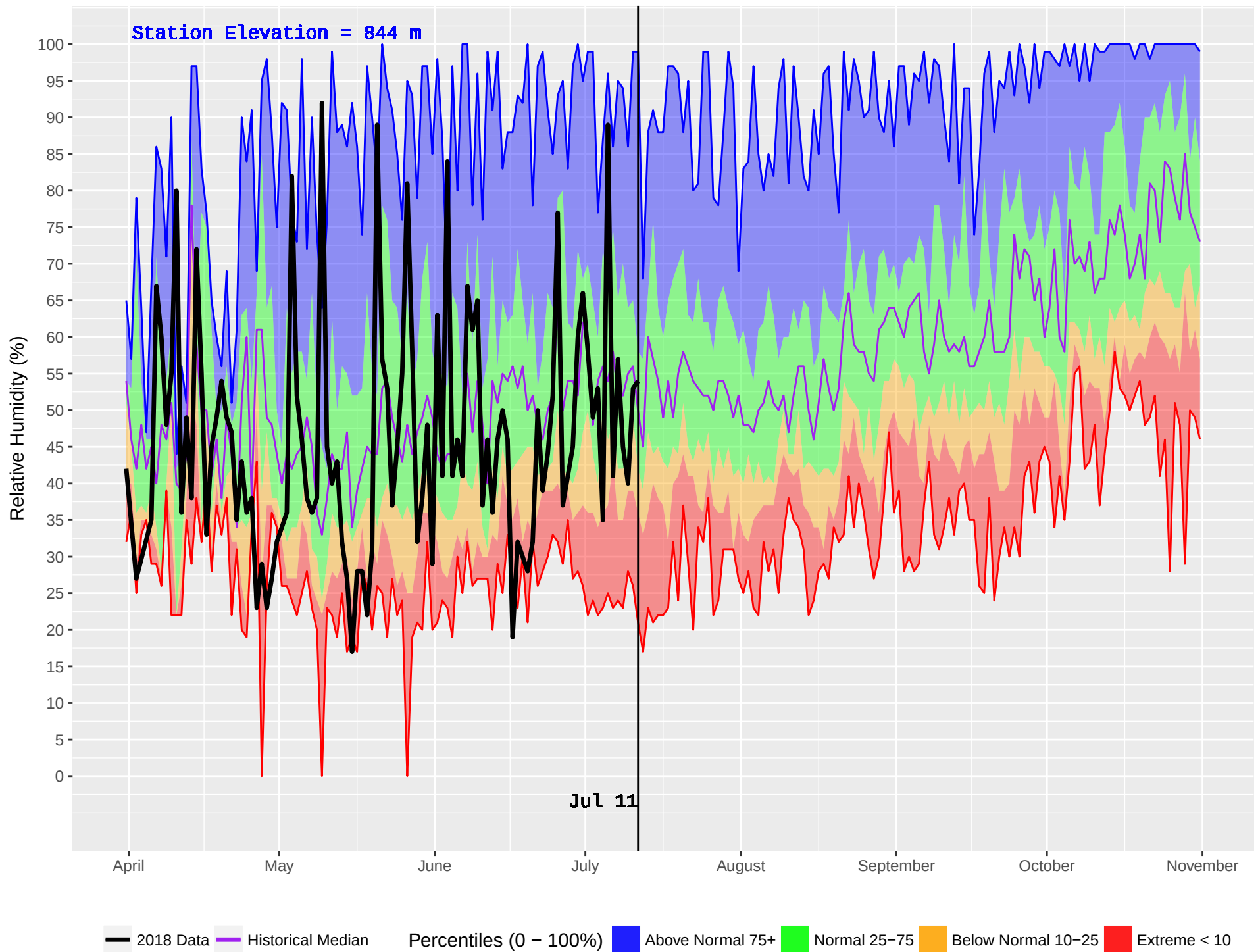
GANOKWA (182) : Historical (1993–2016) and Current (2018) Noon Relative Humidity
